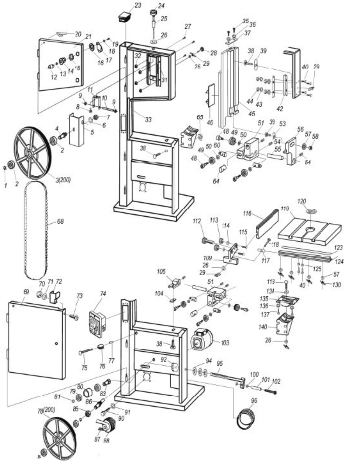
14" (345MM) TWO SPEED BANDSAW BS-345H
